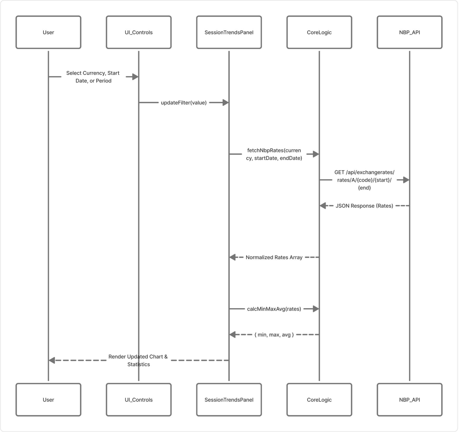
NBP Analytics Sequence Diagram (Updated)
